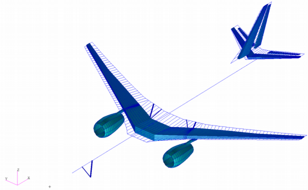
Figure 6: The FE-Model of the XRF1-DLR-C [14]
