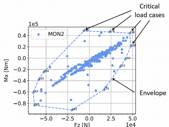
Figure 2: Identification of critical load cases with the classical cutting loads method [4]
