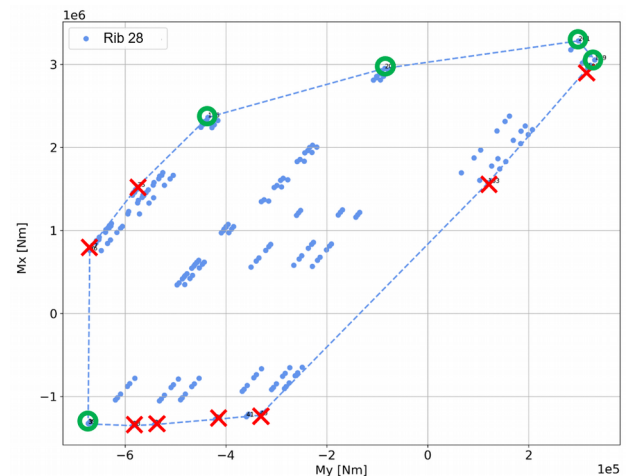
Figure 11: Cutting loads at monitoring station Rib 28, Green mark: Identified by both methods, Red mark: Reduced by the new method
