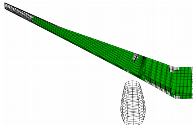
Figure 14: Every element where load case 201 has the highest failure index
