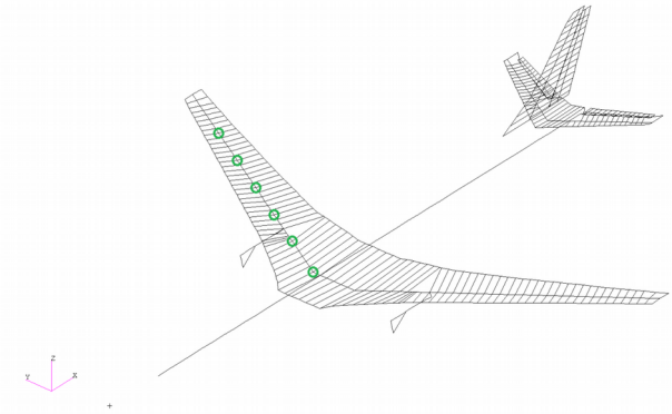
Figure 7: Condensed FE-Model of the XRF1-DLR-C with monitoring stations [14]
