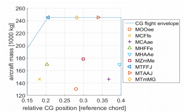
Figure 5: Mass envelope of the XRF1-DLR-C [14]
