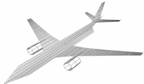
Figure 8: The DLM-Model of the XRF1-DLR-C
