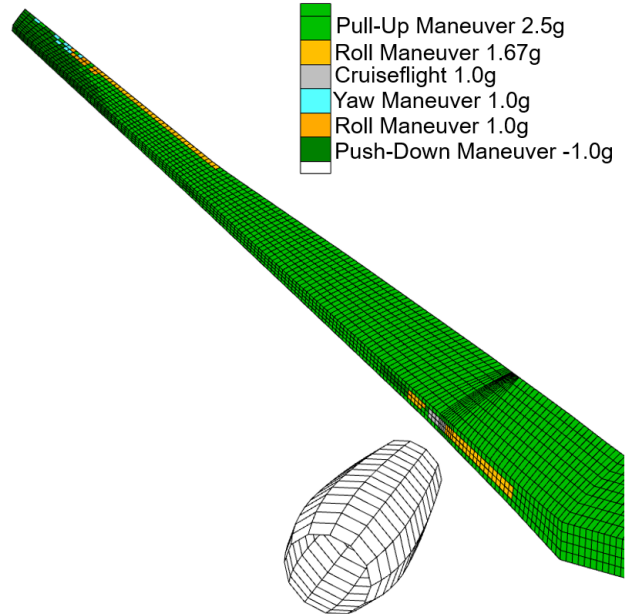
Figure 13: Load cases with the highest failure index for each element
