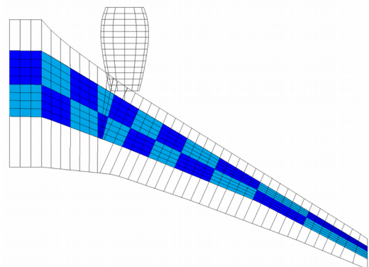
Figure 9: Design fields for the XRF1-DLR-C [14]
