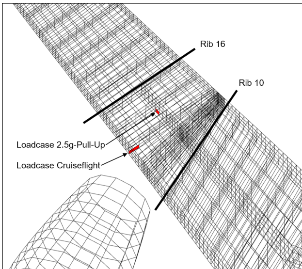
Figure 12: Detailed view of the two additional identified load cases between rib 10 and rib 16
