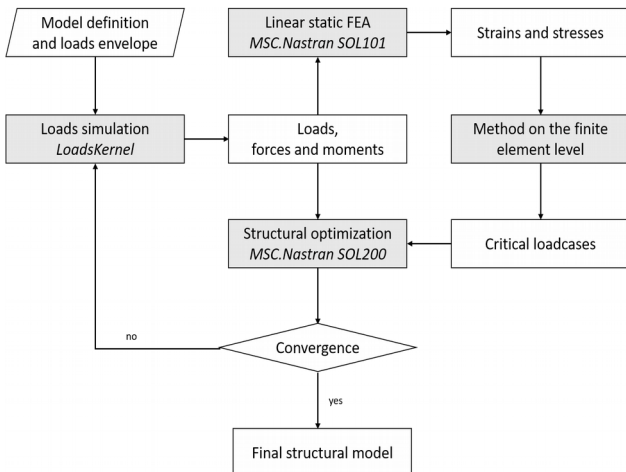
Figure 10: Parametric design process MONA with the method on the finite element level [4]
