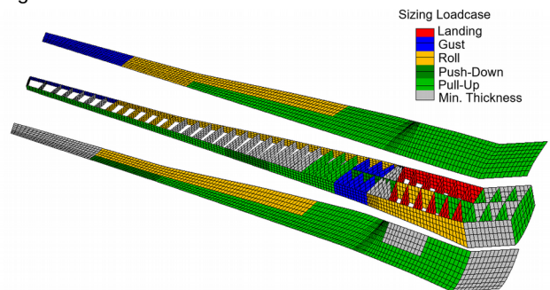
Figure 15: Sizing load cases of a comprehensive load set with landing, gust, and maneuver cases and with maneuver and gust load alleviation
