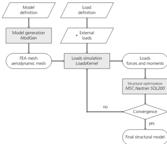
Figure 3: Parametric design process MONA with LoadsKernel [5]
