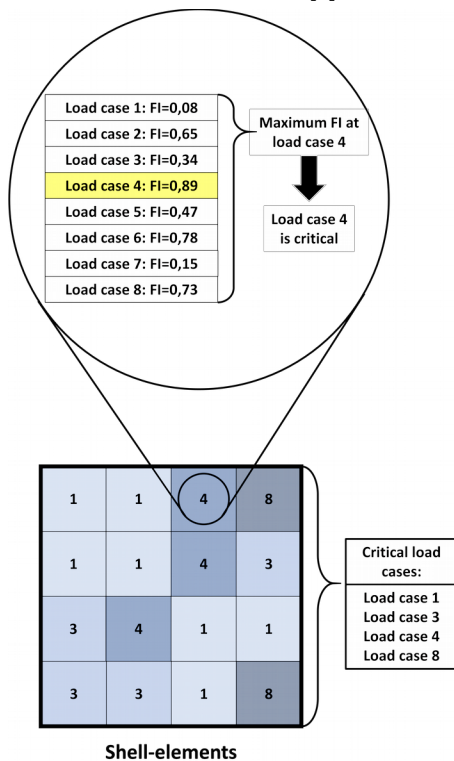
Figure 1: Identification of critical load cases with the new method on the finite element method [4]
