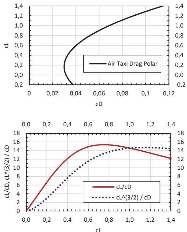
Figure 5 – Aerodynamic Performance
