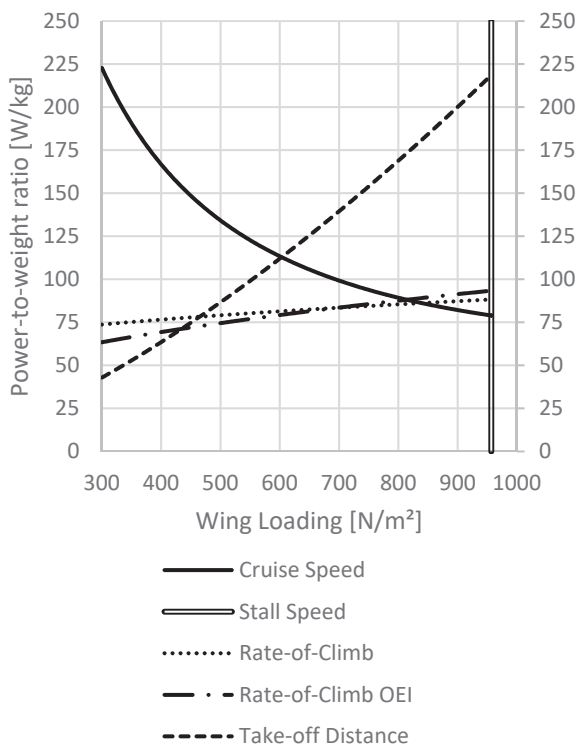
Figure 6 – Matching Diagram (Example)
