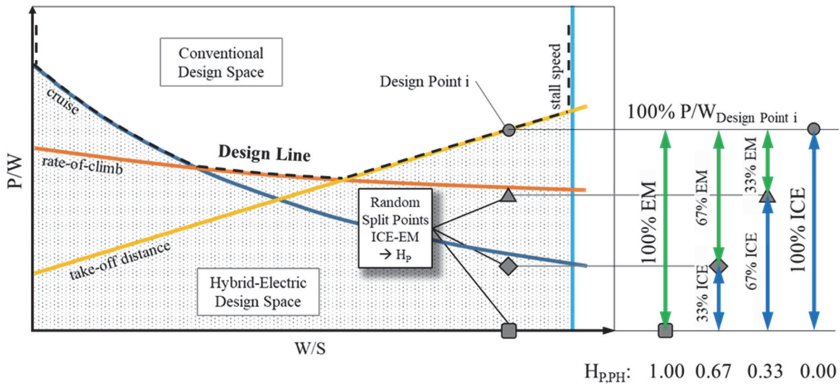
Figure 1 – Matching Diagram for Parallel Hybrid Electric Aircraft
