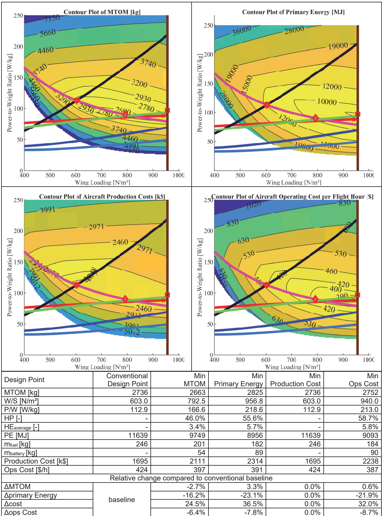
Figure 9 – Sizing Results – 500 Wh/kg Batteries
