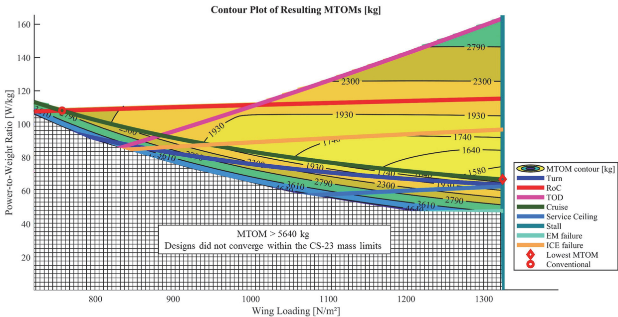
Figure 2 – Thumbprint plot of an Exemplary Design Space Exploration
