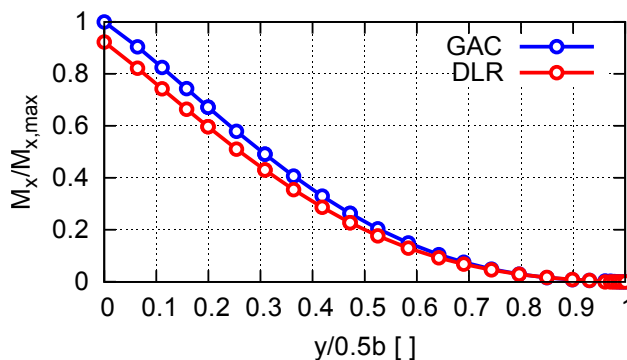
FIGURE 9. Normalized bending moment M_x for the wing for a 2.5 g symmetric maneuver load case
