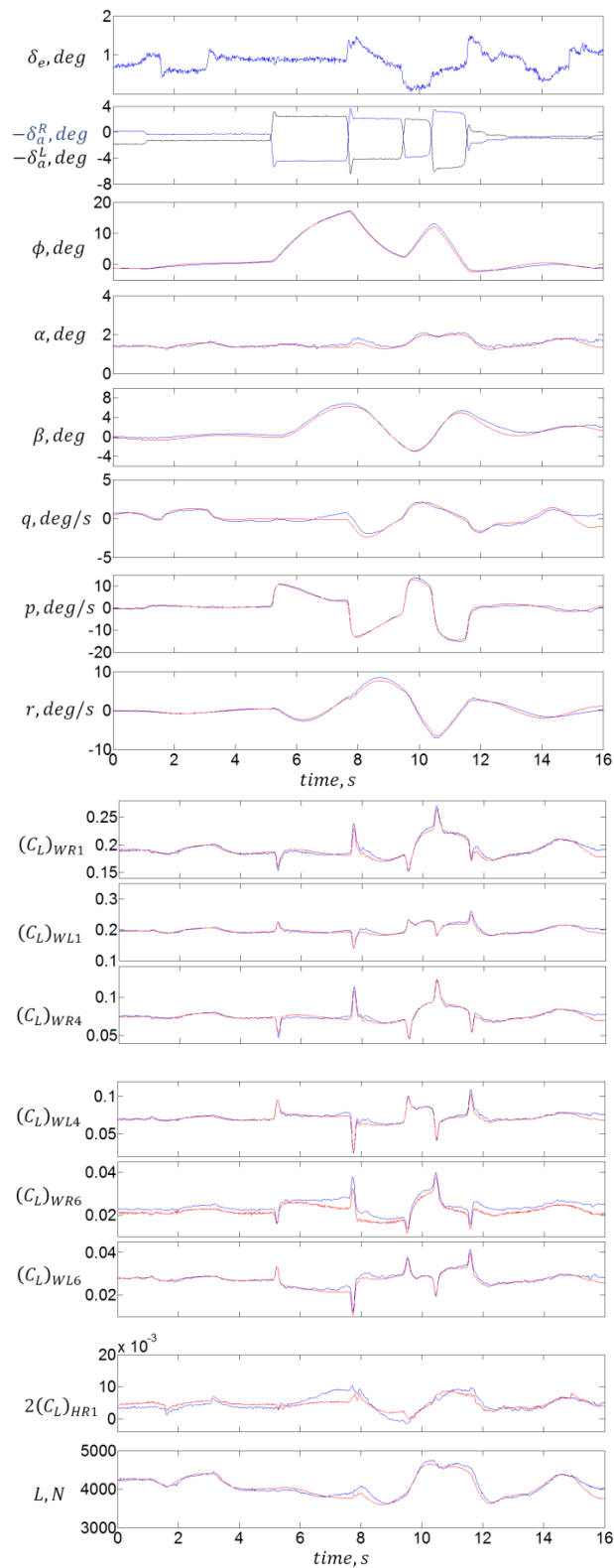
FIGURE 23. Comparison Measurement – Model: 3-2-1-1 aileron multistep inputs
