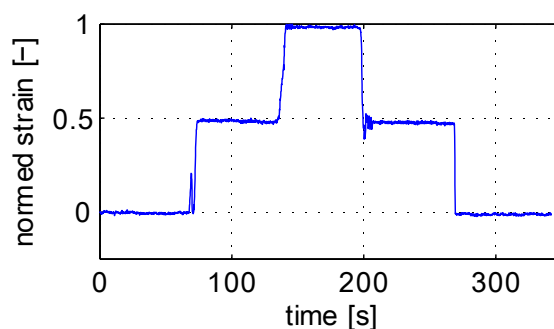
FIGURE 14. Typical strain response of a two-step load application
