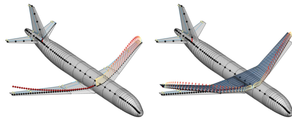
FIGURE 3. Multi-fidelity, physics based disciplinary modules
