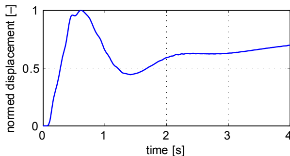
FIGURE 13. Time history of the normed hardpoint displacement from a numerical gust simulation
