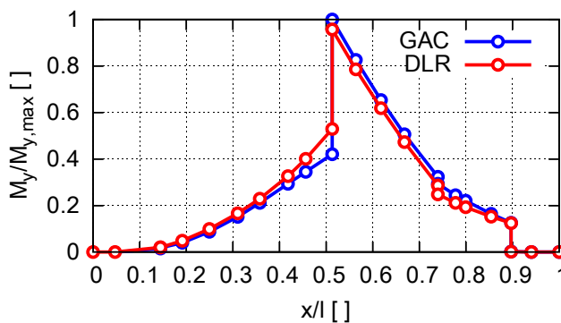
FIGURE 10. Normalized bending moment M_y along the fuselage for a 2.5 g symmetric maneuver load case
