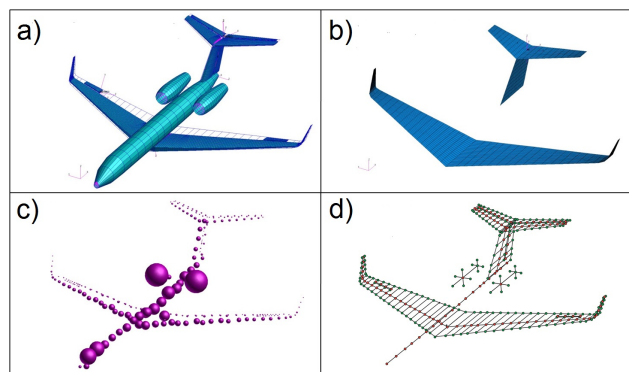
FIGURE 8. Finite element model HALO-S and aerodynamic model for DLM
