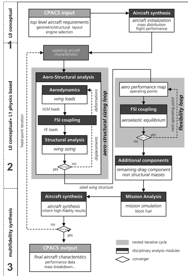
FIGURE 1. Multi-Fidelity Loads Process
