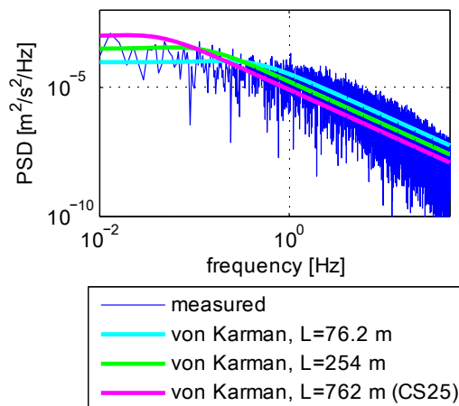
FIGURE 18. Power spectral density of measured turbulence in comparison with reference von-Kármán spectra
