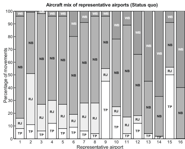
FIG. 4: Daily aircraft mix for 16 representative airport clusters and status quo flight data (based on [11]).
