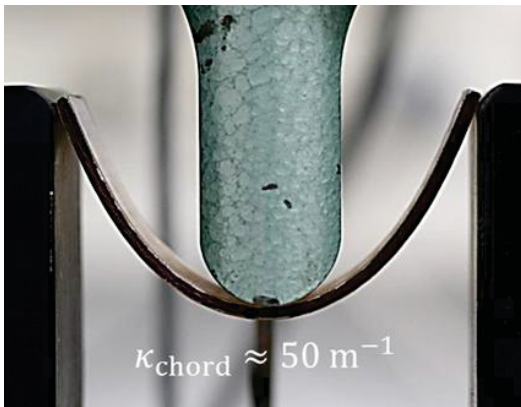
FIGURE 9. Static three-point bending test in chord (0°) direction
