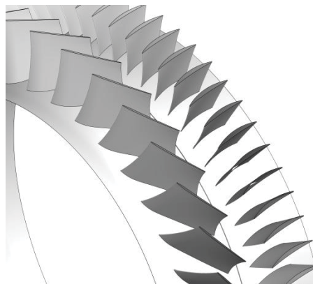
FIGURE 14. Result of optimized preliminary compressor design [24].
