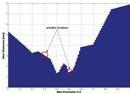
FIGURE 11. Preliminary Results of Variation of Skin Thickness
