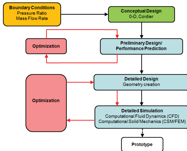
FIGURE 13. Optimization Design Process Chain for the Compressor Design
